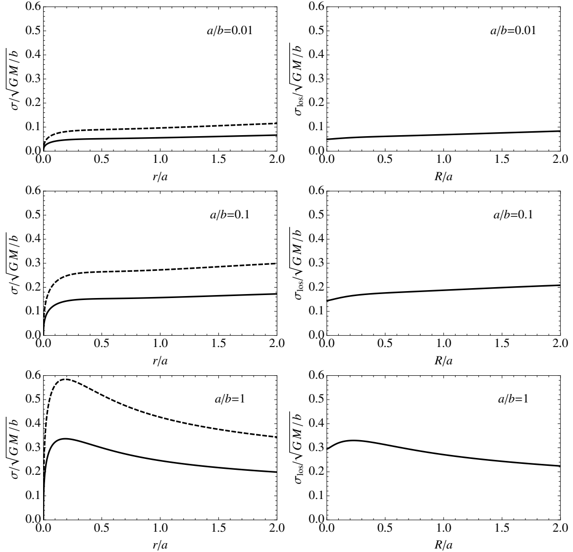
Fig. 2. Velocity dispersion profiles associated to the distribution function presented in Fig. 1 for different degrees of embedding, namely \alpha = a/b = 0.01, 0.1, \text{ and } 1 from top to bottom. Left column: intrinsic radial (solid) and tangential (dashed) velocity dispersions as a function of radial distance r/a . Right column: corresponding line-of-sight velocity dispersions as a function of projected distance R/a . The resulting \sigma_{\text{los}} profiles are relatively flat, especially for small \alpha , i.e., 0.01 and 0.1, and reach a finite value at the center. In general, the curves bear a good resemblance to the observed velocity dispersion profiles of stars in dSph satellites of the Milky Way, as determined in, e.g., Walker et al. (2009).
