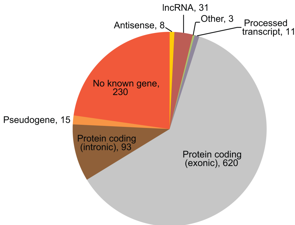
Figure 3. Mapping regions of cis -regulated tags. The gene biotypes and exon/intron locations of unique cis -regulated tags, according to Ensembl v.69 annotation, are shown. The numbers indicate the number of tags mapping in the genes of the corresponding type. doi:10.1371/journal.pgen.1003594.g003
