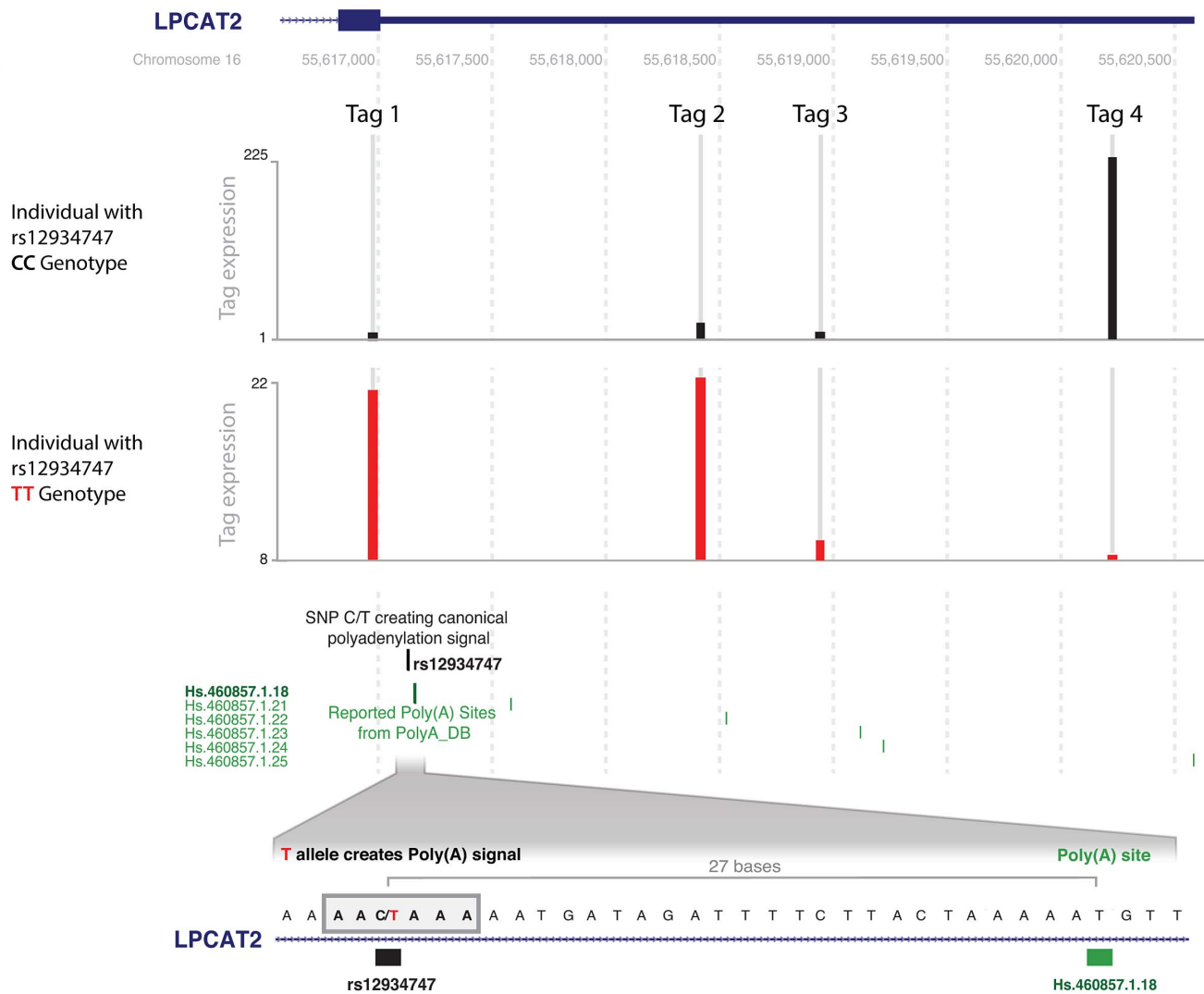
Figure 6. rs12934747*T creates a poly(A) signal in LPCAT2 and leads to alternative polyadenylation site usage. The y-axis represents the number of counts for the deepSAGE tags. Two samples with different genotypes for SNP rs12934747, CC (reference allele) and TT (alternative allele), are shown as different traces. Below the coverage tracks, the position of rs12934747 is shown, together with the position of all reported polyadenylation sites from polyA_DB. An enlargement of the region containing the SNP is shown below. rs12934747 is located at the beginning of the 3'-untranslated region (3'-UTR) of LPCAT2 , 27 nucleotides upstream a reported and experimentally validated polyadenylation site. This SNP changes the sequence, creating a polyadenylation signal that leads to the usage of the reported polyadenylation site. The square block indicates the sequence of the polyadenylation signal created by rs12934747. The creation of this signal shortens the 3'-UTR, as indicated by the higher abundance of the proximal DeepSAGE just upstream of the polyadenylation signal, and the nearly absent distal DeepSAGE, in the sample with the TT genotype (both tags indicated by arrows). Tag 2 was filtered out because it was expressed in less than 90% of individuals. There is an additional tag 3 in-between the proximal and distal tags, which is not cis -regulated. doi:10.1371/journal.pgen.1003594.g006
