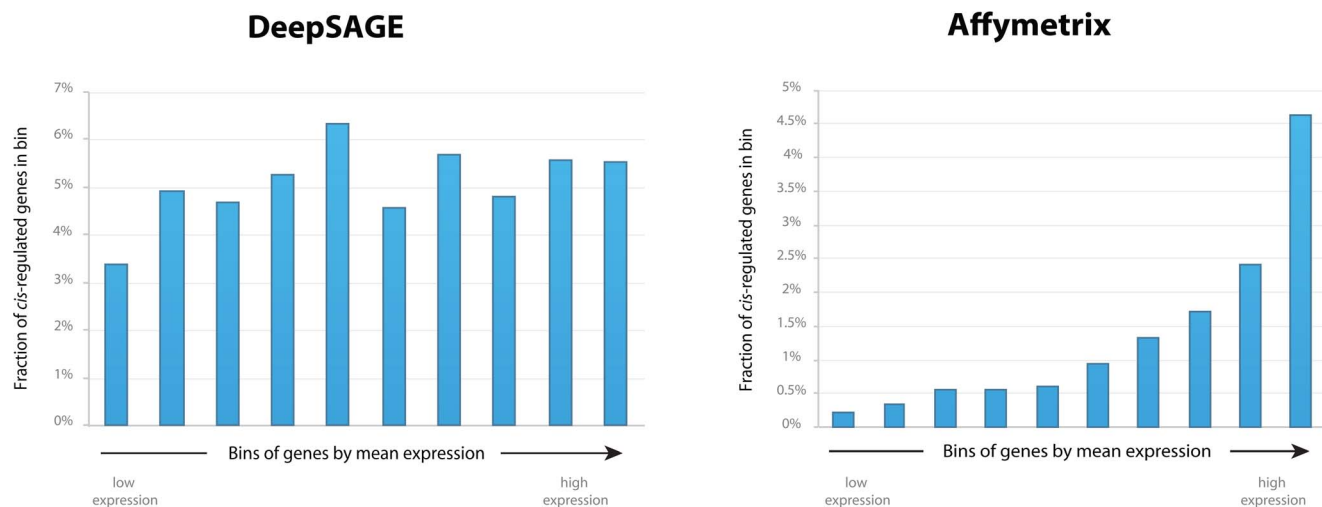
Figure 2. Fraction of cis -regulated genes in bins by mean gene expression levels for DeepSAGE and Affymetrix data. For each dataset, all genes were sorted by their mean gene expression levels, and divided into ten equal bins. The X-axis reflects these bins, which are sorted by increasing mean gene expression levels. The Y-axis reflects the fraction of cis -regulated genes that fall into each bin. doi:10.1371/journal.pgen.1003594.g002
