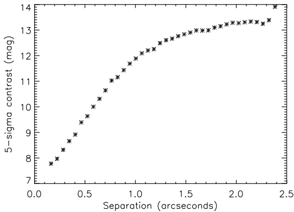
Figure 2. The upper limits on emission from the region surrounding \kappa CrB determined by the Keck AO imaging. This is converted to upper limits on the companion mass in Section 3.2, shown in Fig. 5.
