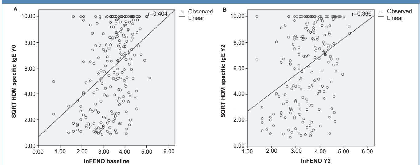
Figure 1. Cross-sectional correlations between fractional expired nitric oxide (FeNO) values and house dust mite (HDM)-specific IgE in the total group (n=251) at (A) baseline and (B) year 2 (Y2) (both p<0.0001). SQRT= square root transformed, ln=ln-transformed
