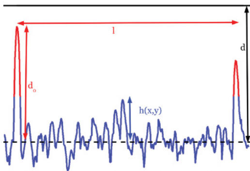
FIG. 5. (Color online) Schematic of a rough surface to clarify the meaning of the parameters l and d_0 . Similar to l , l' represents the distance between the deep troughs, and d'_0 represents the depth of the deepest pit. h(x, y) = h_1(x, y) + h_2(x, y) is the combined surface profile, so that effectively only one rough surface is considered.
