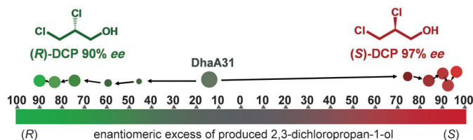
Figure 7. Schematic overview of the obtained evolutionary pathway.
