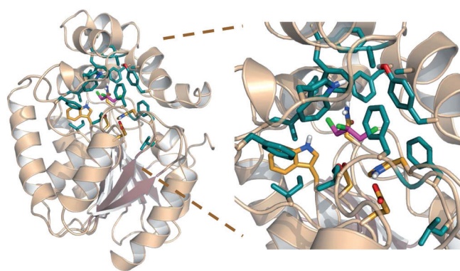
Figure 1. Structural model of DhaA31 with TCP (magenta) docked in the active site. Catalytic residues are displayed in orange and the targeted first-shell residues are displayed in turquoise.
