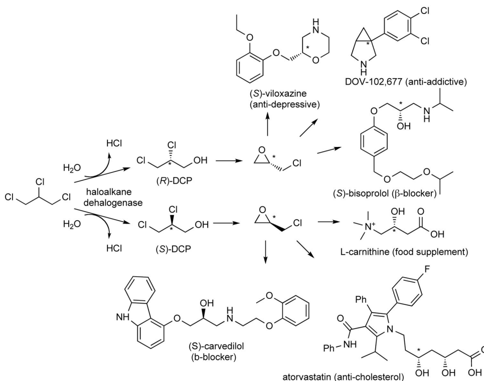
Scheme 1. Desired enantioselective conversion of TCP into ( R )- and ( S )-2,3-dichloropropan-1-ol by enantiocomplementary haloalkane dehalogenase variants. The products can be converted into epichlorohydrins with inversion of configuration at their chiral centers under basic conditions. [26] Both epichlorohydrin enantiomers can be used as intermediates for the production of chiral bioactive compounds.
