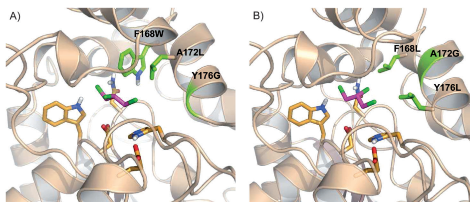
Figure 4. Close-ups of the active sites of the best clones r2-60R (left) and r2-85S (right), after two rounds of evolution. Catalytic residues are in orange, mutated residues in green. Left: Best R -enantioselective variant with three mutations (F168W + A172L + Y176G). TCP is docked in the active site in a configuration that leads to ( R )-2,3-dichloropropan-1-ol formation. Right: Best S -enantioselective variant with different mutations at the same positions (F168L + A172G + Y176L) and with TCP bound in a configuration that leads to S product formation. The positions 168, 172, and 176 presumably have a strong steric effect on the bound substrate in the active site. For modeling see the Experimental Section.
