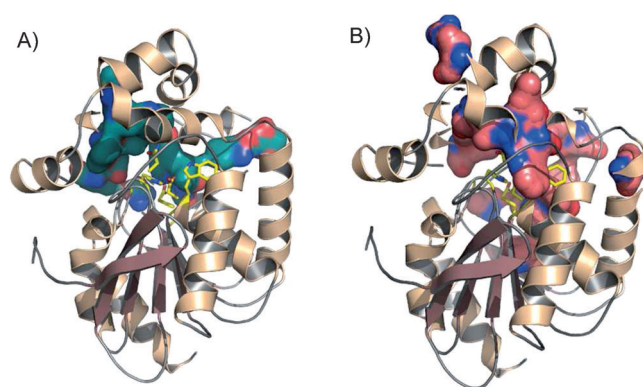
Figure 6. Structural models of the final best enantiocomplementary DhaA variants r5-90R and r5-97S. A) Variant with 13 mutations producing ( R )-DCP. B) Variant with 17 mutations producing ( S )-DCP. The models show the mutated amino acids in surface display revealing the wide distribution. Catalytic residues are shown in yellow.
