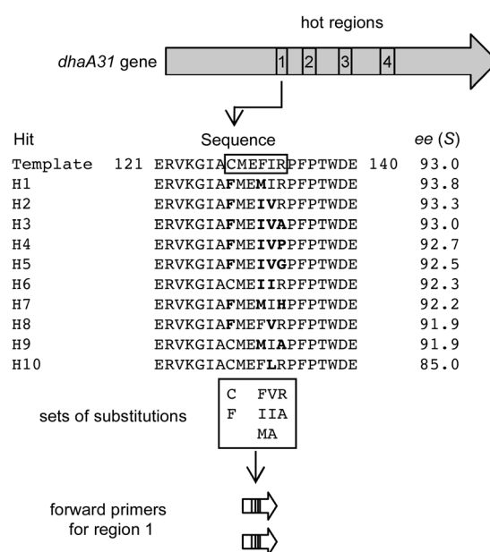
Figure 5. Combinatorial library design for the final round of directed evolution for S -product-selective haloalkane dehalogenase. Four hot regions, each encompassing four to six influential positions, were subjected to site-restricted mutagenesis (SRM). For each position, a restricted set of amino acids was selected on the basis of the mutants from previous rounds. Ten such earlier mutants (H1–H10) are given here, together with their ee values. The restricted sets of amino acids were introduced by QuikChange PCR with use of oligonucleotides or mixtures of oligonucleotides containing partly undefined codons at the target positions. The first hot region, with segment C128–R133 (boxed), for example, is modified to (C/F)ME(F/I/M)(V/I/A)(R/A). The template sequence is the best hit of round 4 (r4-93S, Table 2), and is identical to DhaA31 in the region that is shown.
