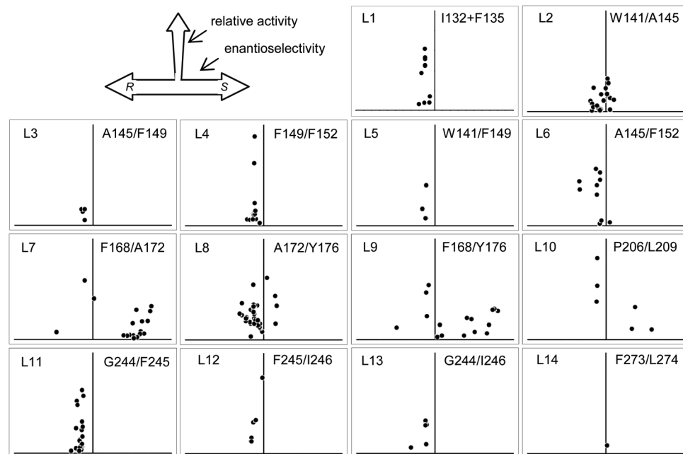
Figure 3. Screening results for 14 first-round mutant libraries. The product ee values (from 100% R to 100% S ) are displayed on the horizontal axes and the relative activities (conversion compared to wild type) are displayed on the vertical axes. Dots indicate individual clones with measurable activity and enantioselectivity.
