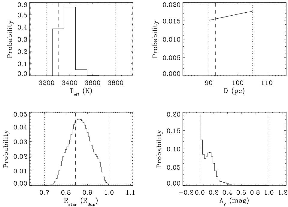
Fig. 5. Bayesian probability distributions for effective temperature T_{\text{eff}} , visual extinction A_V , distance D and stellar radius R_* for ET Cha using our new simultaneous BVRJI photometry (solid histograms). The vertical dotted lines bracket the range of values explored for each parameter while the vertical dashed line represent the absolute best fit photospheric model.
