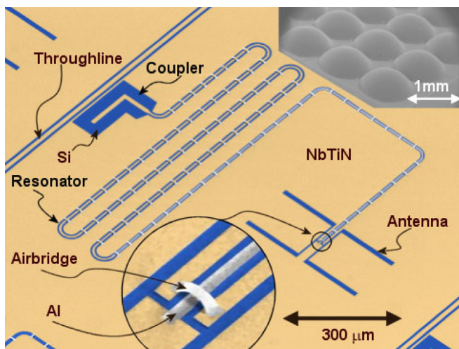
FIG. 1. (Color online) Scanning electron micrograph (SEM) of the hybrid MKIDs used. Indicated is NbTiN, the silicon substrate, and aluminum which is used as the sensitive area of detector and for airbridges. Inset bottom shows the aluminum airbridges. Inset top right is an SEM of a laser machined Si lens array, used to couple radiation via the antenna into the MKID.
