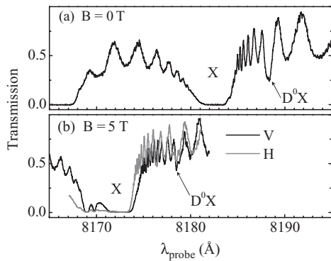
FIG. 6. Scanning-probe transmission spectra taken at B = 0\text{ T} (Reproduced with permission from Sladkov et al. , Phys. Rev. B 82 , 121308(R) (2010). Copyright ©2011 American Physical Society (see Ref. 30) (a) and B = 5\text{ T} (b). Traces were recorded with linear H or V polarization for the probe light (giving identical results at 0 T). For performing these experiments the microscope was defocused to a spot diameter of about 16\mu\text{m} . The strong absorption due to free excitons (X) and much weaker features due to donor-bound excitons ( D^0X ) are labeled. The data at 5 T shows a diamagnetic shift of about 10\text{Å} with respect to the data at 0 T.
