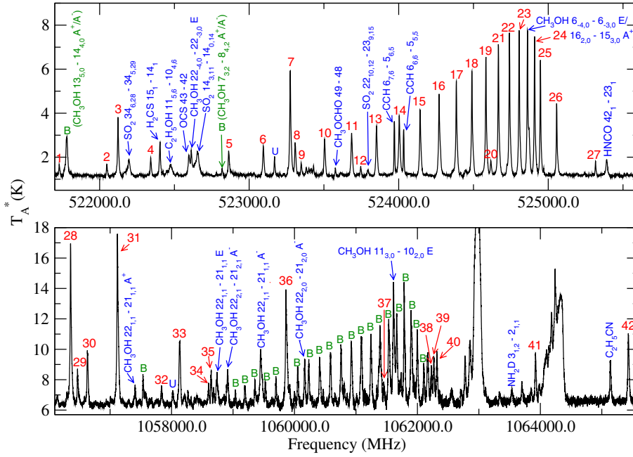
Fig. 1. HIFI spectra of two methanol bands in band 1a (521.7–525.6 GHz; upper panel) and 4b (1056.1–1065.6 GHz; lower panel). Red number 1–42 label isolated methanol transitions, which are also listed in Table 1. Blue texts label transitions from other molecules and the methanol transitions which are blended. Green texts and “B” label the methanol lines which are blended with different parity states. “U” labels two unidentified lines.
