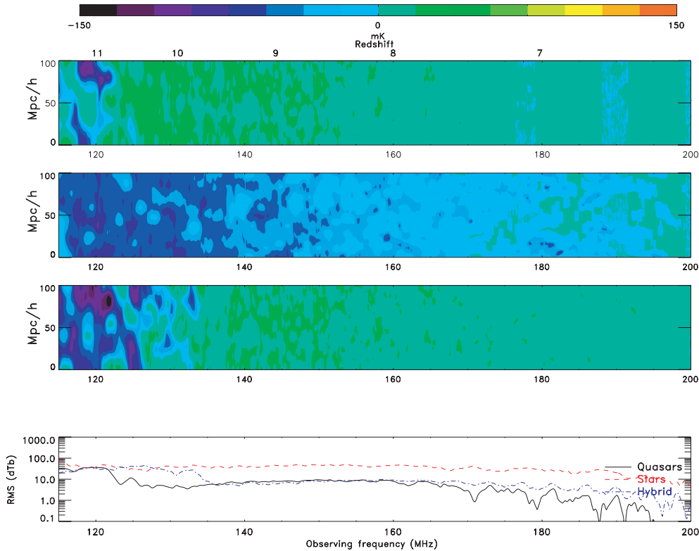
Figure 13. Convolution with LOFAR-PSF. Differential brightness temperatures after convolution with a PSF corresponding to LOFAR is plotted for the same case as in Fig. 11, with the temperatures plotted in mK.
