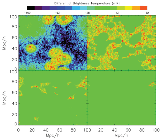
Figure 10. Differential brightness temperature for the hybrid model. Slices correspond to that in Fig. 1. The temperatures (mK) are indicated on a linear scale in the colour bar. The large extent of heating and sufficient J_o ensure that the IGM well beyond the location of the source is rendered visible in 21-cm emission.
