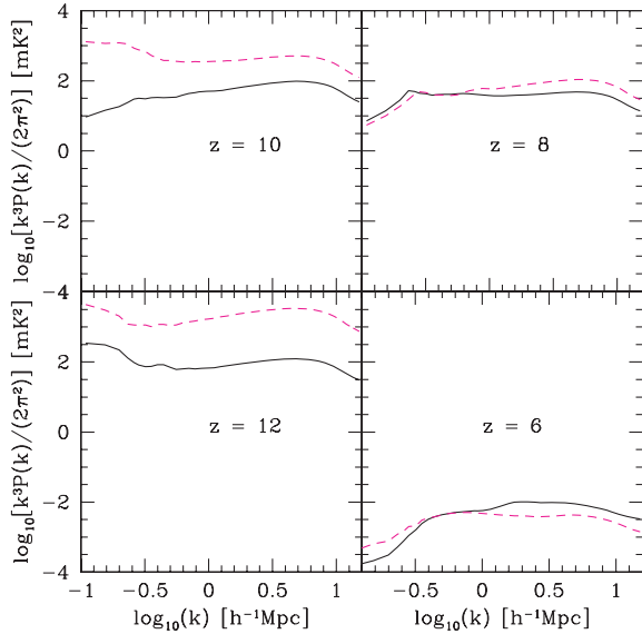
Figure 14. The 3D power spectra of \delta T_b at four different redshifts (as indicated on the panels) are plotted. The solid curves indicate the power spectra resulting from the self-consistent inclusion of T_s and the dashed curve, under the assumption T_s = T_k . At the onset of reionization, z \approx 12 in our model, \delta T_b is larger at all scales under this assumption because we have enforced, in effect, an artificial decoupling of T_s from T_{\text{CMB}} in regions of the simulated Universe where T_k \ll T_{\text{CMB}} . But by redshift 10 the power spectra match exactly as the Ly \alpha becomes efficient everywhere in the box to couple T_s to T_k . Note that the power keeps dropping as x_{\text{HII}} \rightarrow 0 and Universe gets reionized at lower redshifts.
