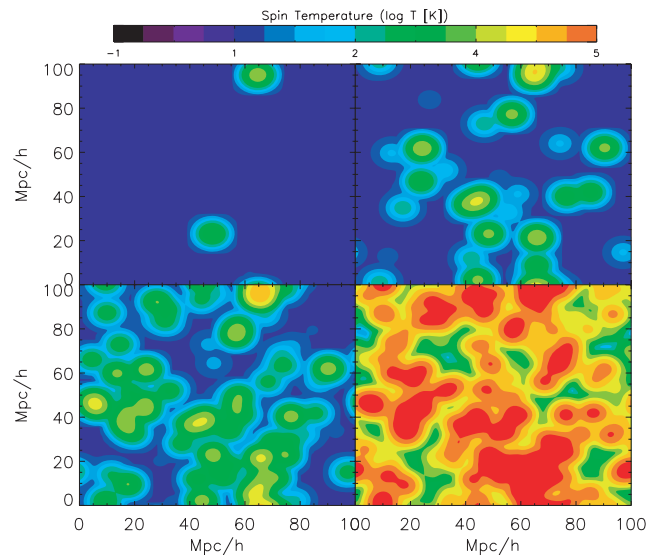
Figure 2. Spin temperature for stellar sources. Slices correspond to that in Fig. 1. Collisional coupling is efficient to couple the T_k to T_s at the centre but the figures also indicate that there is sufficient J_o to couple T_k to T_s well beyond the ionized region, where T_k < T_{\text{CMB}} . The colour bar indicates temperature on a \log T [K] scale.
