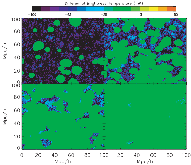
Figure 3. Differential brightness temperature for stellar sources. Slices correspond to that in Fig. 1. The temperature is now contoured on a linear scale with values indicated on the colour bar. In these slices, \delta T_b , starting from zero within ionized regions, attains large negative value outside because stars are not efficient at heating the IGM beyond their ionized bubble and hence cannot render the IGM visible in emission. Early on (top-left) at a redshift of 10, there are only a few sources and the heating induced collisional coupling or the J_o is not high enough to render the Universe visible, but the photons bluewards of \text{Ly}\alpha can reach far outside the ionized region where they are injected into \text{Ly}\alpha frequency causing substantial coupling to the kinetic temperature which is much below the CMB. At later times, the ionized bubbles overlap significantly driving the brightness temperature to zero.
