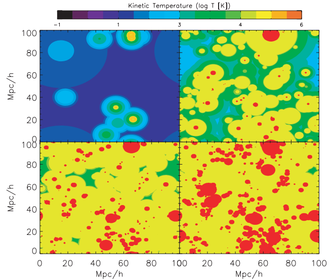
Figure 8. Kinetic temperature for hybrid model. Slices correspond to that in Fig. 1, with temperatures indicated on a \log T [K] scale. The heating pattern is peculiar in that the temperature shows a much ‘cuspier’ behaviour towards the centre. The reason is that the stellar component of the source ionized the very central part and the X-ray radiation can thus heat the central part to even higher temperature. On the other hand the large extent of the heating is attributed to the power-law component of the SED.
