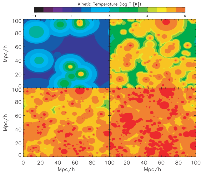
Figure 4. Kinetic temperature for mini-QSO sources. Slices correspond to that in Fig. 1 with temperatures indicated on a \log T [K] scale. Here, we see the striking difference between mini-QSOs and stars in the extent of heating. The amplitude is about \approx 10^{6.5} K towards the centre and spatial extent of the heating is about a few Mpc. Already at redshift 10 (top-left) the average temperature is of the order 10^3 K.
