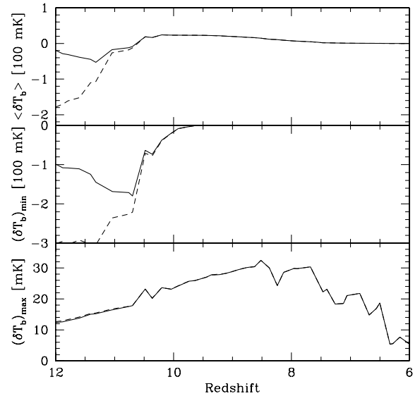
Figure 15. Plotted are the mean (top), minimum (middle) and maximum (bottom) values of \delta T_b as a function of redshift. Line styles correspond to Fig. 14. Because at earlier redshifts (around 12) T_k \ll T_{\text{CMB}} within a large fraction in the simulation box, the minimum value attained by assuming T_s = T_k is much lower than when only regions with Ly \alpha excitation (which is typically near the source) is allowed to couple T_s with T_k . For the same reason, the maximum value in both cases is similar because the assumption holds close to the sources as the presence of Ly \alpha flux ensures efficient coupling. As a result the global average \delta T_b is also lower for the approximated model at the onset of reionization and catches up quickly to the ‘proper’ model as the Universe fills up with sufficient Ly \alpha flux.
