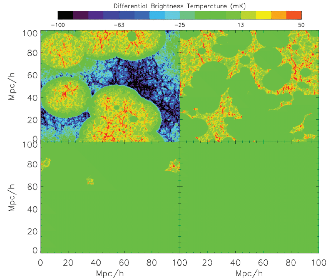
Figure 6. Differential brightness temperature for mini-QSO sources. Slices correspond to that in Fig. 1. Note here that the brightness temperature (mK) is plotted on a linear scale with values as indicated on the colour bar. We see again from the top-left panel that although the number of sources in the field are few, they were efficient in both increasing T_k dramatically and providing sufficient J_o to ‘light-up’ the Universe in 21-cm around them. The spheres in the top-left panel have \delta T_b of zero because they are highly ionized.
