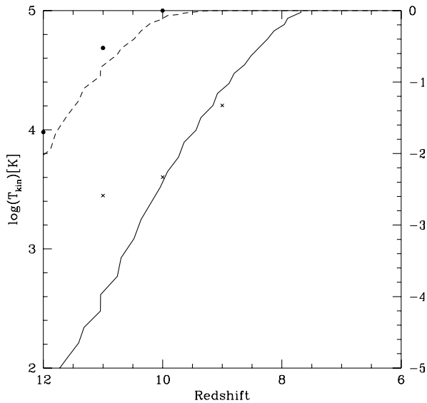
Figure 18. Plotted here are the evolution of the gas temperature T_k (solid line) and the volume filling factor (dashed line) of the X-ray radiation as a function of redshift for the case of the mini-QSOs. For comparison, points from Santos et al. (2008) are shown for T_k (crosses) and filling factor (filled hexagons) with their case of f_x = 10 and photon energies 100.0 eV.
