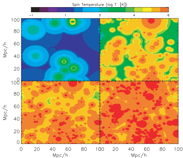
Figure 5. Spin temperature for mini-QSO sources. Slices correspond to that in Fig. 1 with the temperatures indicated on a \log T [K] scale. Spin temperatures show an interesting ring-like behaviour (easily visible in the top-left panel). The reason for this is discussed in the text.
