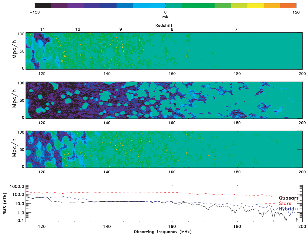
Figure 11. Contrasting reionization histories. From the top, reionization histories ( \delta T_b in mK as a function of frequency or redshift) are plotted for mini-QSO, stellar and hybrid sources, respectively. The bottom panel plots the rms of \delta T_b as a function of redshift/frequency for all the three cases.
