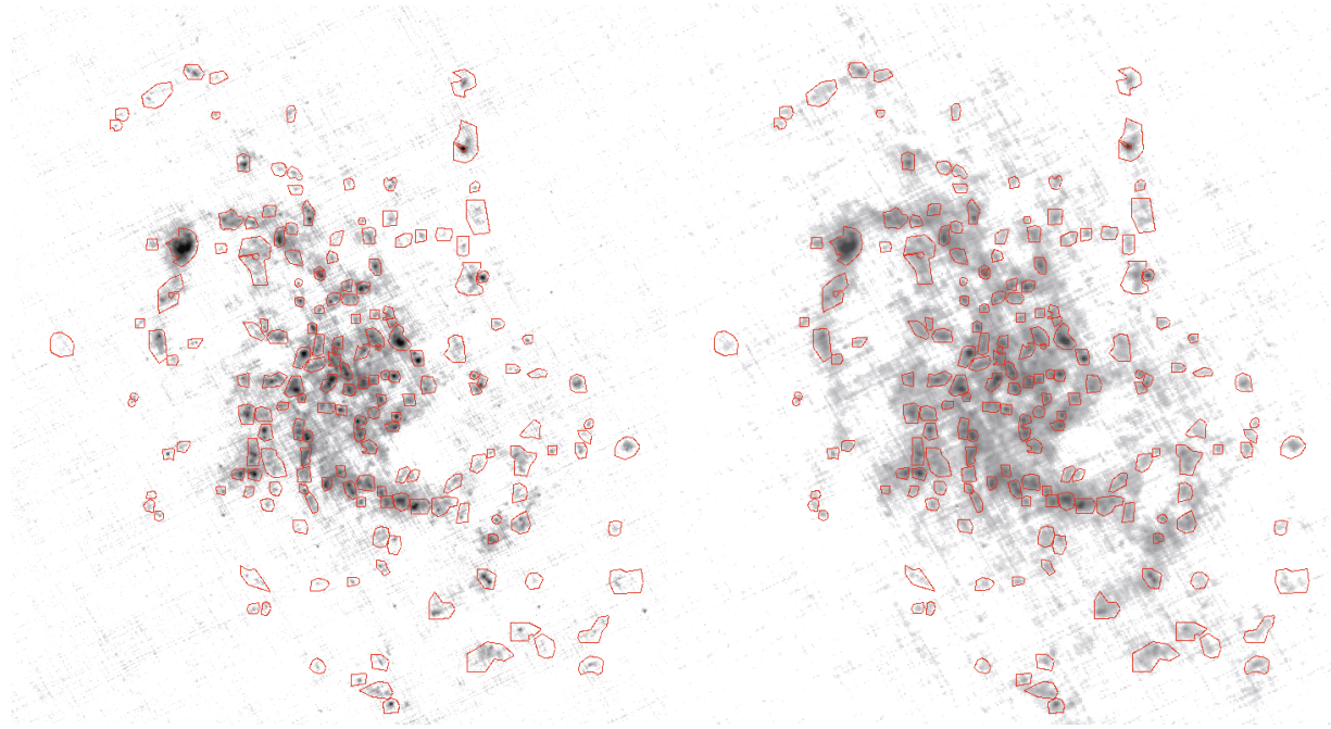
Fig. 1. PACS maps of M 33 at 100\ \mu\text{m} (left) and 160\ \mu\text{m} (right). To probe the full dynamic range of the image a logarithmic scale is used. Individual clumps are well resolved with minimal blending. Some diffuse emission is visible, particularly in the arms and the central region of the galaxy. The visible perpendicular stripes in each scanning direction are sampling artefacts. The red polygons represent the selected apertures. North is up, East is left.
