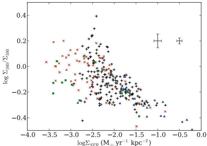
Fig. 3. \Sigma_{160}/\Sigma_{100} vs. \Sigma_{SFR} (black pluses), for the 179 HII regions selected in M33. The error bars correspond to the typical uncertainty for the lower and higher 50% percentile. For comparison additional entire galaxies are plotted using the same colour scheme as in Fig. 2.
