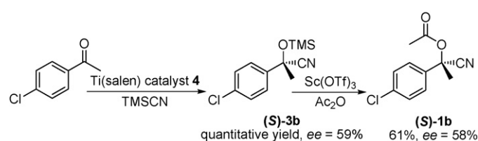
Fig. 2. Ketone-derived cyanohydrin acetates tested in the hydrolysis.
