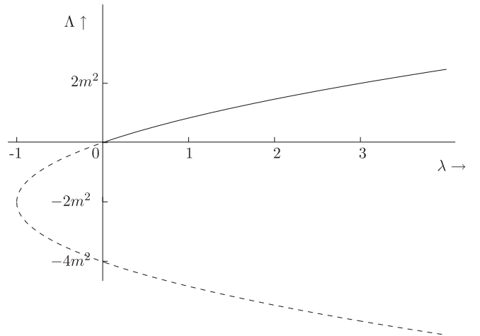
FIG. 2. The case \sigma = 1 , m^2 > 0 , with the dashed line indicating the region with positive central charge. There is no region with unitary gravitons.
