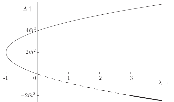
FIG. 3. The case \sigma = 1 , m^2 < 0 , with the thick line indicating the region consistent with the BF-type bound, and the dashed line the region with positive central charge.
