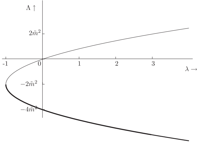
FIG. 4. The case \sigma = -1 , m^2 < 0 , where the thick line indicates the region consistent with the BF-type bound, while there is no region with positive central charge.
