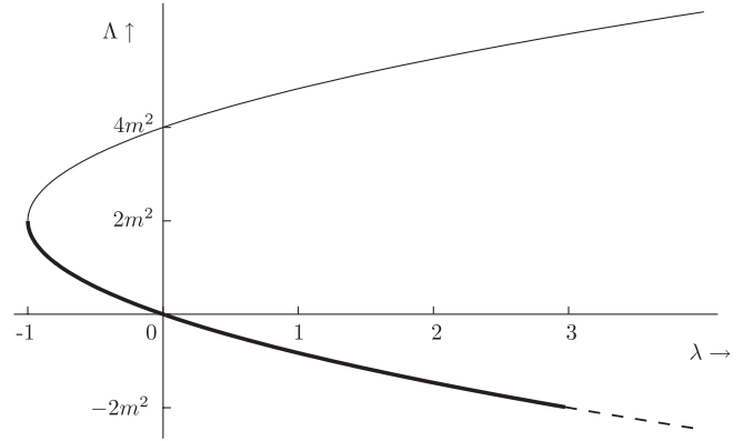
FIG. 1. The case \sigma = -1 , m^2 > 0 , where the thick line indicates the unitary region, and the dashed line the region with positive central charge.
