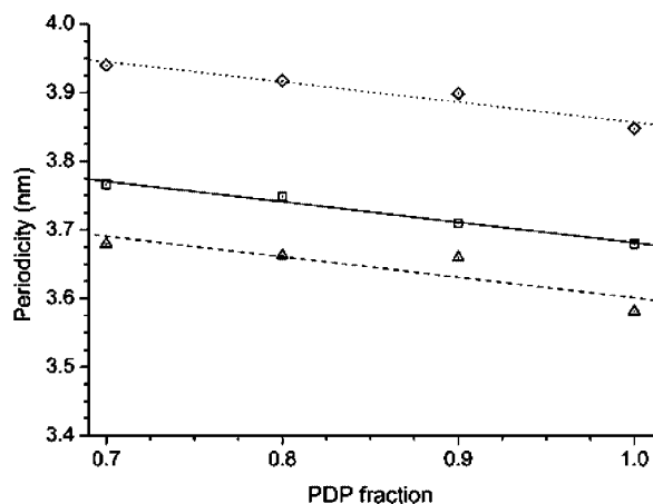
Figure 7. Periodicity of P4VP(PDP) x samples as a function of the fraction PDP: (□) 5 °C below T_{ODT} ; (◇) below ODT at 30 °C; (△) above ODT at 70 °C, corresponding to the correlation hole peak.
