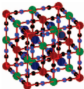
Figure 1. Representation of the unit cell of \text{RbMn}[\text{Fe}(\text{CN})_6] \cdot z\text{H}_2\text{O} . 20
