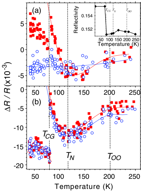
FIG. 3 (color online). Temperature dependence of transient reflectivity probed at 4 ps ( \circ ) and 100 ps ( \blacksquare ) for excitation power densities of (a) 85 mJ/cm 2 and (b) 190 mJ/cm 2 . Lines are guides for the eye. Inset shows stationary reflectance calculated using the optical constants taken from Ref. [18].
