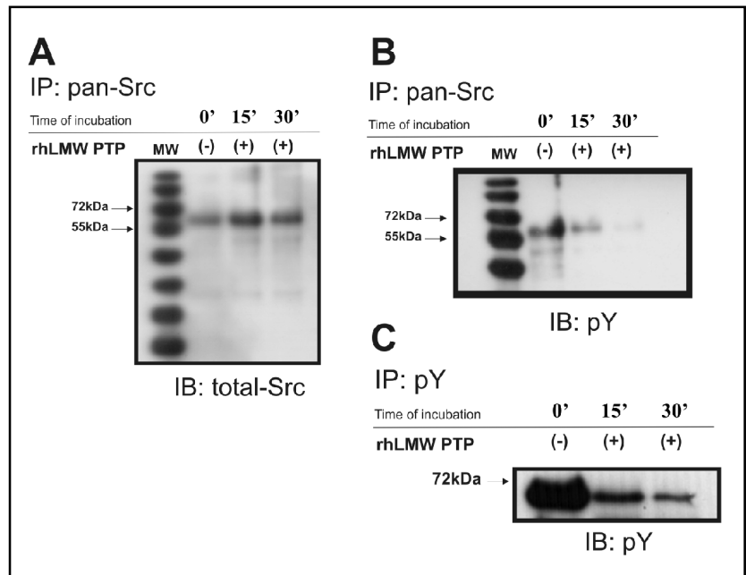
Fig. 2. LMWPTP dephosphorylates Src at tyrosine residues. Cells were pretreated with pervanadate for 30 min (to increase pY-Src levels) and pan-Src (i.e. non-phosphorylated and phosphorylated-Src) was immunoprecipitated and incubated with rhLMWPTP in vitro for different lengths of time. (A) Equal amounts of pan-Src were used in the various experimental conditions, as assessed by western blotting with a pan-Src antibody (left panel). MW = molecular weight marker lane. (B) Western blots of immunoprecipitated rhLMWPTP-treated Src probed with pY antibodies. (C) Western blots of immunoprecipitated rhLMWPTP-treated Src probed with \alpha -pY antibodies.
