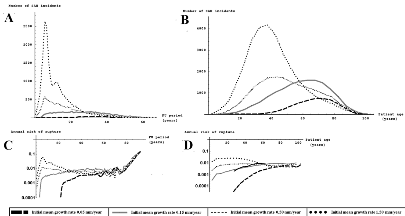
FIG. 3. Graphs depicting the number of SAH incidents during follow-up (A) and as function of patient age (B). Graphs illustrating the annual risk of rupture, on a logarithmic scale, during follow-up (C) and as a function of patient age (D), for 4 illustrative IMGRs. The solid black line in panel D represents the annual SAH incidence rates derived from the literature. FU = follow-up.
