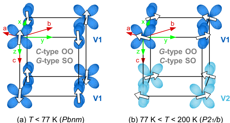
Figure 1. Orbital and spin ordering patterns in \text{YVO}_3 for (a) T_S < 77 K and (b) T_S < T < T_{OO} = 200 K [15], [21]–[32]. The xy orbital is occupied by one electron on each site (not shown). The occupation of xz and yz orbitals is C -type below T_S and G -type above (see main text for more details). SO is lost at T_N = 116 K. The coordinates of the Pbnm and P2_1/b crystal systems are given in the upper left corner of each figure.
