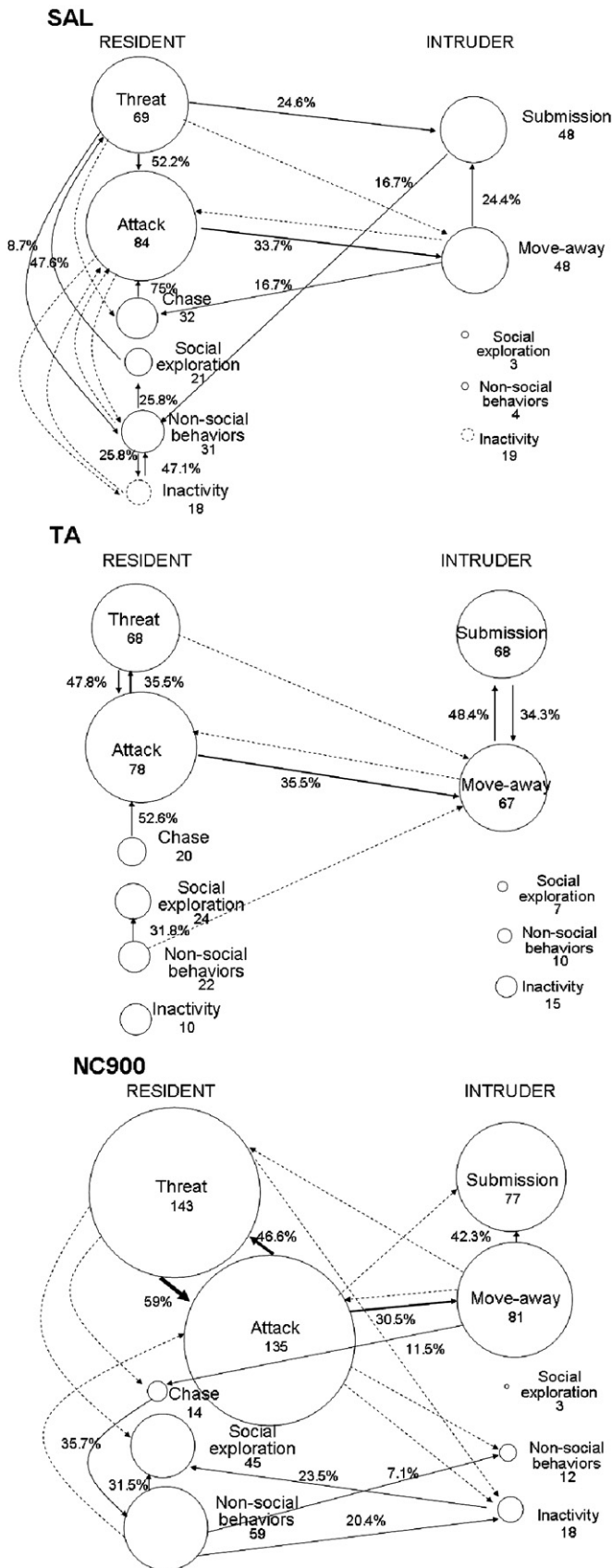
Fig. 4. Kinestogram of behavioural transitions performed in the first minute after the first attack of the last male–male resident-intruder confrontation (R19) by male mice from the aggressive lines (SAL, TA and NC900). The areas of circles
