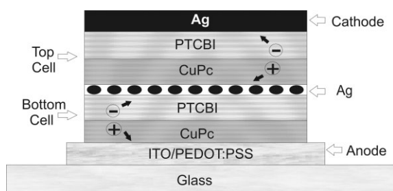
Figure 2. The structure of an organic tandem solar cell based on the small molecules CuPc (donor) and PTCBI (acceptor), as described earlier. [24]. The 0.5 nm Ag separation layer provides recombination sites for the free charges arriving from the bottom and top cell.
