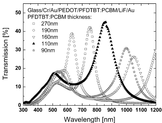
Figure 9. The optical transmission through the bottom cell for different thicknesses of the active layer of the device. At thickness 110 nm, the transmission matches the absorption of the top cell at 850 nm.
