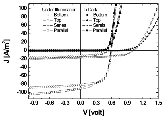
Figure 13. J-V characteristics of the bottom and top cell measured separately, and the tandem cells connected in series and in parallel in the dark and under illumination with simulated solar light of 1000 \text{ W m}^{-2} . In the series configuration, the current density is limited by the lowest current density of the two cells and the V_{OC} is the sum of both sub-cells. In the parallel configuration, the current density is equal to the sum of both sub-cells and the V_{OC} is limited to the lowest V_{OC} of the sub-cells.
