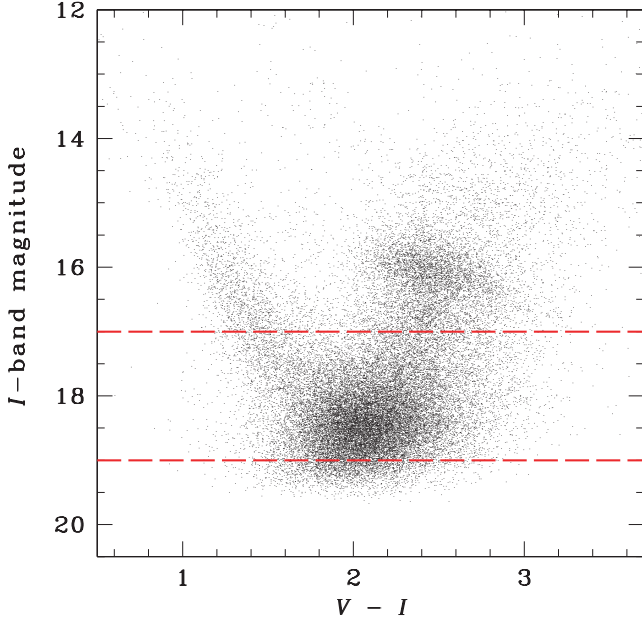
Figure 2. The observed OGLE-II colour–magnitude diagram for field sc3. Note that this is the observed field and not a simulated field, since we do not include V -band data in our simulations. The horizontal lines show the cuts for all events ( I_{\text{out}} < 19 ) and bright events ( I_{\text{out}} < 17 ). The latter sample corresponds to a brightness cut similar to that employed for red clump-giant microlensing events; for this figure, the red clump region is centred around V - I \approx 2.4 , I \approx 16 . In reality, a red clump sample would be selected using a cut in colour to remove foreground blue disc stars, but this is not necessary in our case since our simulation contains no colour information and is set up so that all stars belong to the bulge.
