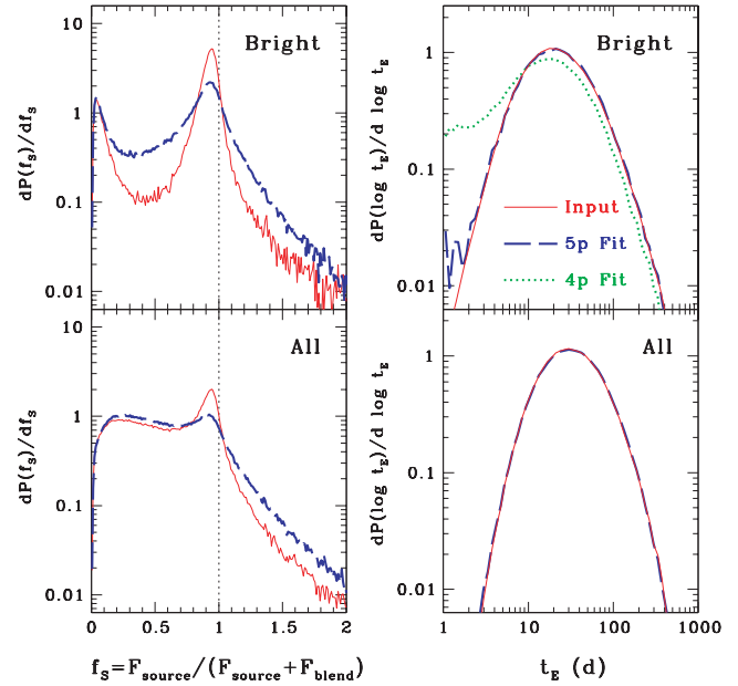
Figure 5. Input and fitted event parameter distributions for the blending fraction (left-hand panel) and the event time-scale (right-hand panel). This figure corresponds to the simulated field with medium stellar density and seeing; the other fields show qualitatively similar behaviour. The solid line represents the input event parameter distribution, the long dashed line represents the five-parameter fit (i.e. unconstrained blending) and the dotted line represents the four-parameter fit (i.e. f_S = 1 ). The top panels show the distributions for a subset of bright events ( I_{\text{out}} < 17 ), such as red clump giants, and the bottom panels show the distributions for all events (i.e. I_{\text{out}} < 19 ). The fitted time-scale distributions in the upper panel are corrected for the detection efficiency and the solid line denotes the underlying time-scale distribution; the lower panel simply shows the distributions of input and fitted time-scales for the detected events (note that since the two distributions in this panel are almost identical, the two lines are coincident).
