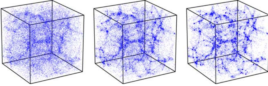
Figure C2. Evolution of galaxy distribution in the Voronoi kinematic model. A sequel of three consecutive time-steps within the kinematic Voronoi cell formation process, proceeding from left to right, and from top to bottom. The depicted boxes have a size of 100 h^{-1} Mpc. Within these cubic volumes some 64 Voronoi cells with a typical size of 25 h^{-1} Mpc delineate the cosmic framework around which some 32 000 galaxies have aggregated. Taken from a total (periodic) cubic ‘simulation’ volume of 200 h^{-1} Mpc containing 268 235 ‘galaxies’.
