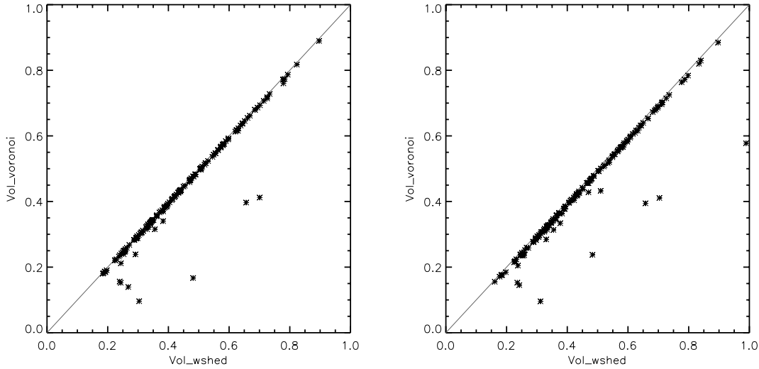
Figure 11. Scatter diagram plotting the WVF void segment volumes against the intrinsic geometric Voronoi cell volume. The solid line is the linear 1–1 relation. Left-hand frame: low-noise Voronoi clustering model. Right-hand frame: noisy Voronoi clustering model.
