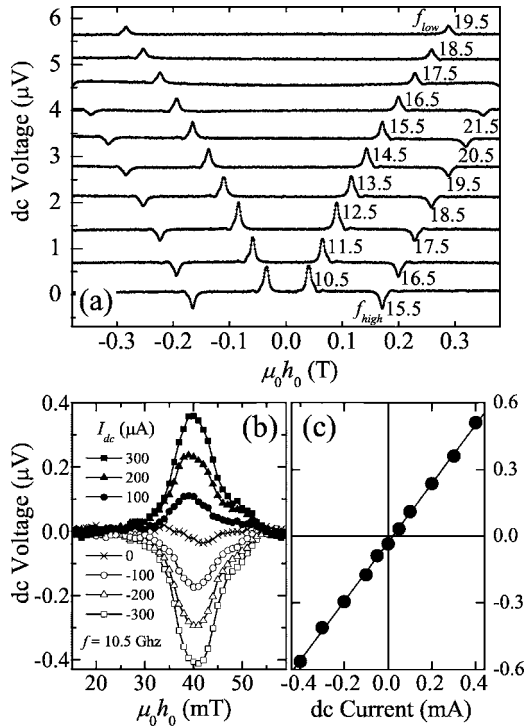
FIG. 2. (a) dc voltage measured at I_{\text{dc}}=400 \mu\text{A} as a function of h_0 using the frequency modulation technique, where each curve represents V=V(f_{\text{high}})-V(f_{\text{low}}) , with f_{\text{low,high}} increasing in 1 GHz increments, and f_{\text{high}}-f_{\text{low}} always 5 GHz. The curves are offset by 700 nV for clarity. (b) The peak at f_{\text{low}}=10.5 GHz for a number of currents between -300 and 300 \mu\text{A} . (c) The peak height from the data in (b) plotted vs the current. The line is a linear fit to the data.
