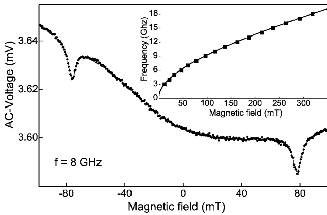
FIG. 2. Measured ac voltage as a function of static magnetic field for an applied rf magnetic field at frequency of 8 GHz. The inset shows the static magnetic field dependence of the resonance frequency, as derived from the dips in the ac voltage vs magnetic field. The squares represent the experimental data, the curve is a fit to the data; using the Kittel formula.
