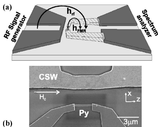
FIG. 1. (a) Schematic diagram of the device. On the left side a rf current is driven through the shorted end of the coplanar strip, which generates a rf magnetic field h_{\text{rf}} (Biot-Savart law). On the right, a loop that contains a submicron Py strip is connected to another coplanar strip. rf power that results from oscillating magnetic flux in this loop is measured with a spectrum analyzer. Magnetization precession of the Py strip contributes a magnetic field h_{\text{FMR}} to the total magnetic field. (b) Scanning electron microscope picture of central part of the device (rotated by 90^\circ with respect to the upper figure).
