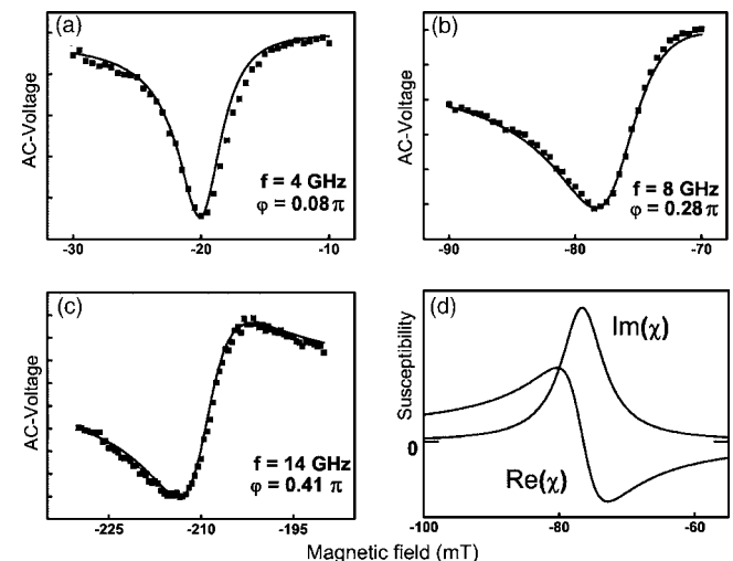
FIG. 4. [(a), (b), and (c)] Measured ac voltage as a function of the static magnetic field, around the resonance position for the frequencies of 4, 8, and 14 GHz, shown by squares. The line is the fit to the data using Eq. (3) (with the value for \phi in the plot). (d) The real and imaginary parts of the susceptibility \chi calculated using Eq. (2) for rf field frequency of 8 GHz, \gamma = 176 GHz/T, M_S = 1 T, and \alpha = 0.015 .
