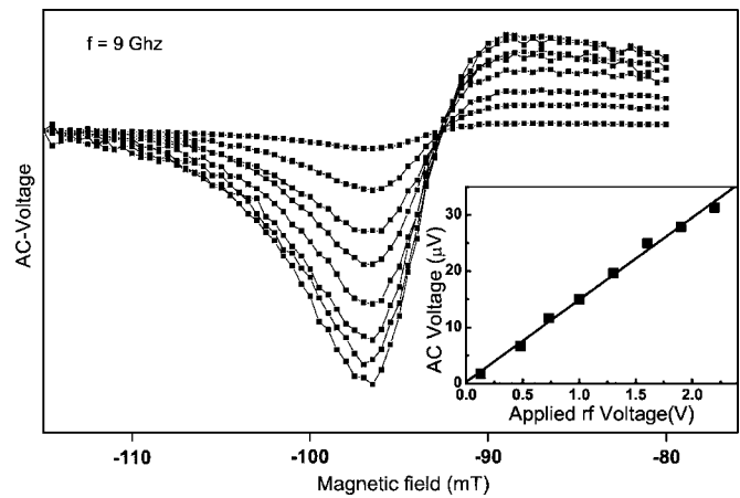
FIG. 3. Measured ac voltage as a function of static magnetic field for a sequence of amplitudes of the rf driving field at 9 GHz. The inset shows a linear dependence for the amplitude of the FMR signature in the measured ac voltage on the amplitude of the driving field (applied rf voltage scale is used, derived from the applied power assuming 50 Ω load impedance).
