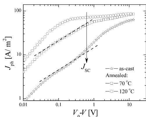
Figure 1. Experimental photocurrent ( J_{ph} ) versus effective applied voltage ( V_0 - V ) of the P3HT:PCBM devices at room temperature for as-cast devices and after thermally annealing of the photoactive layers (see legend). The thickness of the devices ( L ) is 96 nm and the arrow indicates the position of the short-circuit current ( J_{SC} ). The dashed lines represent the square-root dependence of the J_{ph} on voltage.
