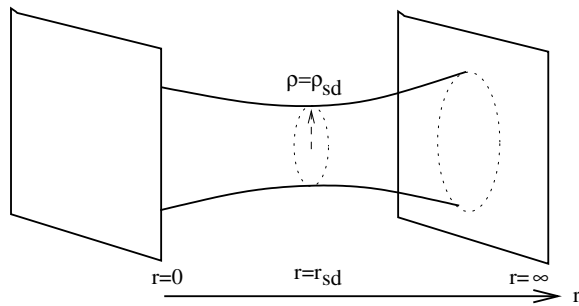
Fig. 1 The geometry of a wormhole. The two asymptotically flat regions at r = 0 and r = \infty are connected via a neck with a minimal physical radius \rho_{sd} at the self-dual radius r_{sd} .
