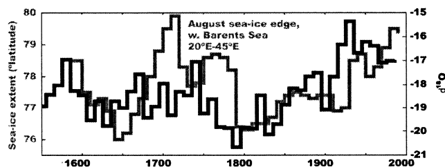
Figure 6 The decadal-scale Austfonna \delta^{18}\text{O} record (black) corresponds well to the August sea-ice record (grey) from western Barents Sea, compiled with data from whaling ships (Vinje, 2001). This suggests that \delta^{18}\text{O} in the precipitation is directly influenced by distance from moisture source in the Austfonna ice-core (from Isaksson et al. , 2003)
