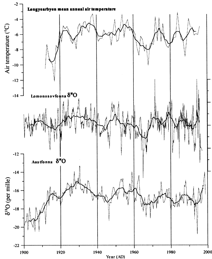
Figure 2 The \delta^{18}\text{O} records from Lomonosovfonna and Austfonna from the twentieth century are compared with the mean annual temperature records from Longyearbyen (Nordli et al. , 1996). The grey line is the unsmoothed data and the black line the running mean for an equivalent of 5 years (from Isaksson et al. , 2003)
