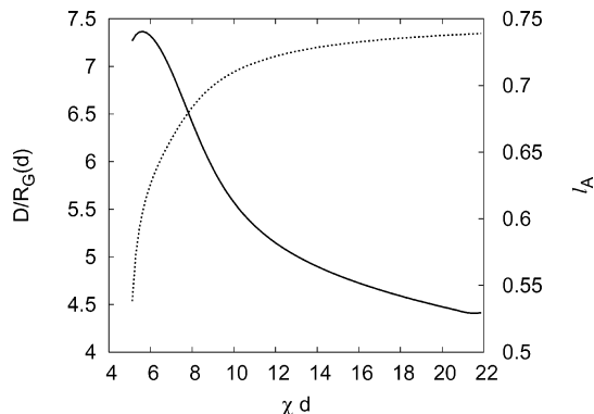
Figure 9. Period D and relative thickness I_A of the A-domain as a function of \chi d of the lamellar structure of the symmetric linear-alternating block copolymer A_4\text{-}b\text{-(B-}b\text{-}A)_2 . D is expressed in units of the radius of gyration R_G = R_G(d) . The solid line corresponds to the periodicity of the lamellar structure, and the dotted line corresponds to the relative thickness of the A-domain.
