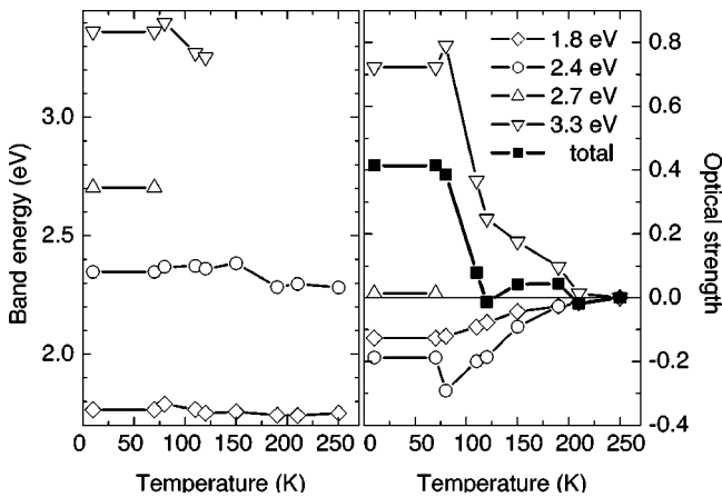
FIG. 12. Temperature dependence of the position of the electron bands (left) and their optical strength together with the total spectral weight of the three bands (right).
