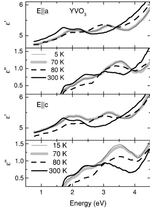
FIG. 8. Real and imaginary parts of the dielectric function for the a and c axes of \text{YVO}_3 .
