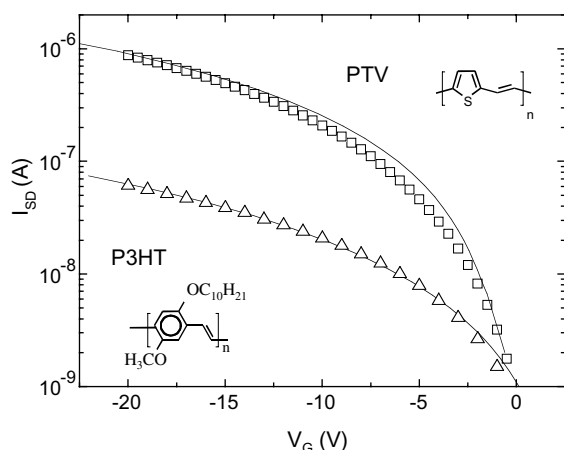
Fig. 2. Drain current versus gate voltage of a PTV and P3HT field-effect transistor for room temperature (taken at a drain voltage of -2 V). The calculated drain currents (Eq. (7)) are indicated by solid lines. The insets show the chemical structures of PTV and P3HT.
