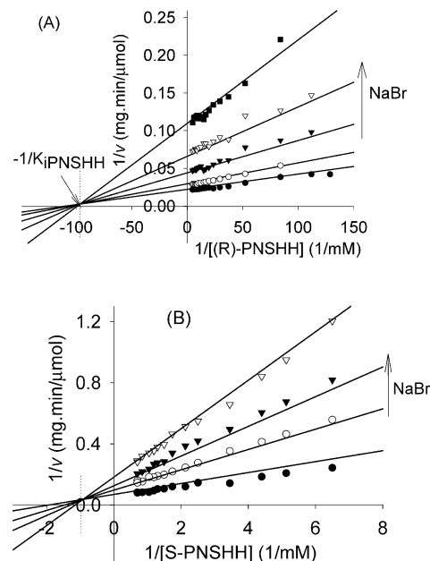
FIGURE 3: Inhibition of HheC by bromide. Panel A: double-reciprocal plots of bromide inhibition on the ring-closure reaction of ( R )-PNSHH. ( R )-PNSHH was varied from 0.007 to 0.1 mM at fixed concentrations of bromide: ●, 0 mM; ○, 0.25 mM; ▼, 0.75 mM; ▽, 1.5 mM; and ■, 3 mM. Panel B: double-reciprocal plots of bromide inhibition on the ring-closure reaction of ( S )-PNSHH. ( S )-PNSHH was varied from 0.1 to 1.6 mM at fixed concentrations of bromide: ●, 0 mM; ○, 0.5 mM; ▼, 1 mM; and ▽, 2 mM. The points are the experimentally determined values; the lines indicate the best fit to these data using eq 2.
