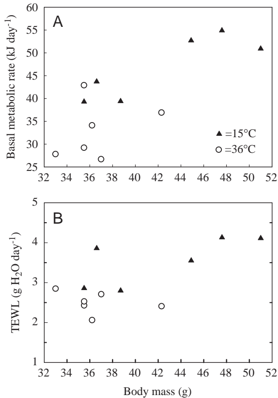
Fig. 1. (A) The relationship between basal metabolic rate ( \text{kJ day}^{-1} ) and body mass (g) in hoopoe larks from the Arabian desert. Filled triangles represent birds acclimated to 15^\circ\text{C} ; open circles represent birds acclimated to 36^\circ\text{C} . (B) The relationship between total evaporative water loss (TEWL; \text{g H}_2\text{O day}^{-1} ) and body mass (g) in hoopoe larks from the Arabian desert. Symbols as in A.
