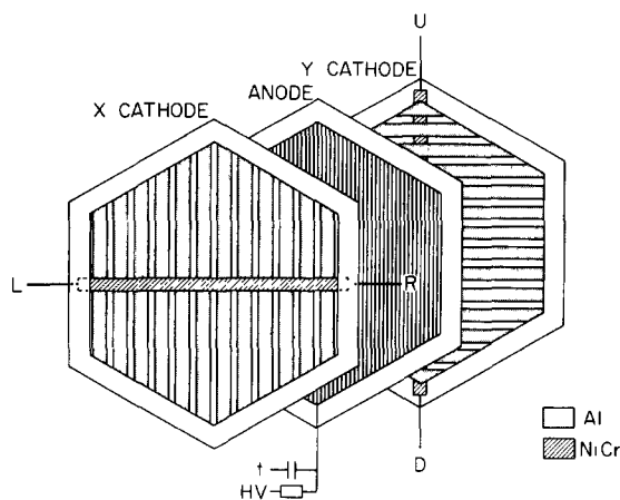
Fig. 3. Exploded view of the hexagonal MWPC.
