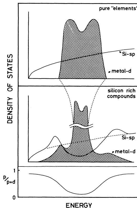
FIG. 6. Schematic illustration of the electronic structure of TM silicides. The upper frame indicates the DOS of the elements without mutual interaction. In the lower frame the effects of the interaction are shown. See text for explanation.
