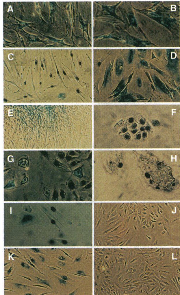
FIG. 1. β-Gal in cultured human cells. Cells were radiolabeled, stained, and photographed at 100× (A–E and J–L) or 200× (F–I) magnification (final magnifications: A–E and J–L, ×60; F–I, ×120). Most cells were either labeled and SA-β-Gal negative or unlabeled and SA-β-Gal positive. Double positive cells comprised <0.1% of early, and 5–8% of late, passage cultures. Such cells may have completed their last cell cycle and induced SA-β-Gal during the 3-day labeling or induced SA-β-Gal before the last cell cycle. Double negatives comprised 1–2% of early, and 20–25% of late, passage cultures. Some were slow-cycling cells, because labeling for 5–7 days reduced them from 22% to 16% and increased labeled cells from 15% to 20%. Others expressed low SA-β-Gal, since longer staining (24 vs. 8 hr) decreased them from 23% to 17% and increased SA-β-Gal positives from 69% to 75%. Ten to 15% of cells in senescent cultures were unlabeled and SA-β-Gal negative for unknown reasons. (A and B) Early passage (A) and senescent (B) WI-38 cells stained for lysosomal β-Gal. (C) Early passage HCA2 cells; labeled, SA-β-Gal staining. An unlabeled SA-β-Gal-positive cell is in the lower right. (D) Senescent HCA2; labeled, SA-β-Gal staining. A labeled SA-β-Gal-negative cell is in upper left. (E) Presenescent, confluent WI-38; SA-β-Gal staining. Staining disappeared 2 days after replating. (F) Early passage NHEK; labeled, SA-β-Gal staining. (G) Middle passage NHEK; labeled, SA-β-Gal staining. (H) Early passage differentiated NHEK; labeled, SA-β-Gal staining. (I) CMV-MJ cells 10 passages after receiving human chromosome 1; labeled, SA-β-Gal staining. Unlabeled SA-β-Gal-positive cells were not seen in the parent culture. (J) IDH4 cells growing in dex; SA-β-Gal staining. (K) IDH4 minus dex for 17 days; SA-β-Gal staining. (L) IDH4 minus dex for 20 days, then plus dex for 3 days; SA-β-Gal staining.
