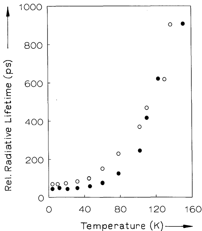
Fig. 2. Relative radiative decay time as a function of temperature for the blue ( \bullet , \lambda_{\max} = 570.2 nm at 1.5 K) and red ( \circ , \lambda_{\max} = 576.1 nm at 1.5 K) excitonic J-bands of PIC-Br aggregates. Excitation was performed at 545 nm
