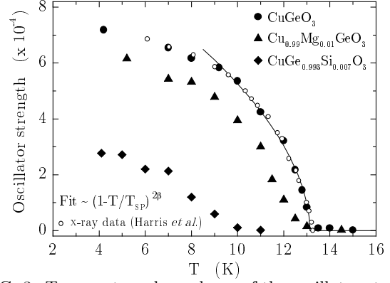
FIG. 3. Temperature dependence of the oscillator strength of the zone boundary mode observed for E||b at 800 \text{ cm}^{-1} on pure (filled circles), 1% Mg-doped (triangles) and 0.7% Si-doped (diamonds) \text{CuGeO}_3 single crystals. For comparison the x-ray scattering data of Harris et al. (Ref. 14) are also plotted (open circles).
