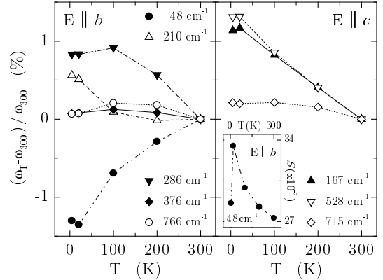
FIG. 4. Temperature dependence of the frequency shift (in per cent) of the transverse optical phonons observed for E||b and E||c on the pure single-crystal of \text{CuGeO}_3 . In the inset the oscillator strength S of the mode detected at 48 \text{ cm}^{-1} , for E||b , is plotted versus the temperature.
