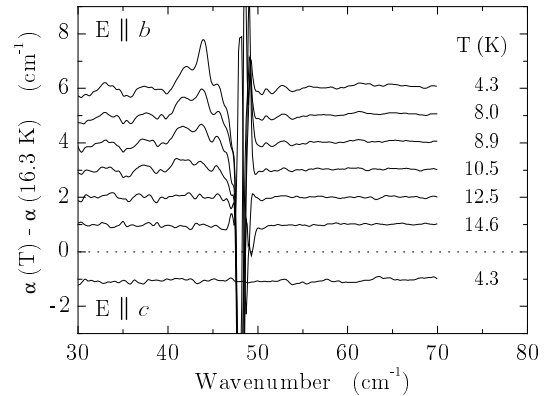
FIG. 5. Absorbance difference spectra for the pure single-crystal of \text{CuGeO}_3 , with E||b and E||c . The spectra have been shifted for clarity.
