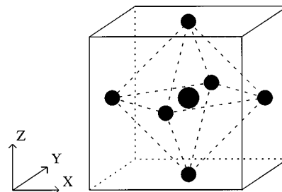
FIG. 1. Cubic perovskitelike crystal structure. The small spheres at the centers of the cubes faces represent oxygen atoms, the large sphere in the center of the cube represents a tungsten atom.
