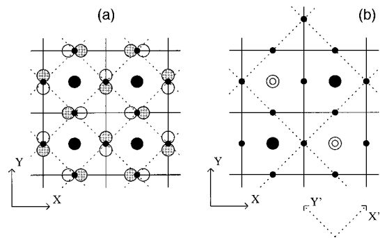
FIG. 3. (a) One of the states at the top of the valence band ( M ) in the simple cubic structure. Solid lines separate a sc unit cell from its periodic images. The dotted lines connect nearest-neighbor oxygen atoms in the x - y plane. The W and O are represented by large and small bullets respectively. (b) Relation between the tetragonal and simple cubic structure. In the tetragonal structure the W represented by two concentric circles have moved into the positive z direction, whereas those represented by the filled circles have moved in the opposite direction. The unit cell contains two formula units and is separated from its periodic images by the dashed lines. Note that it is rotated by 45^\circ around the z axis.
