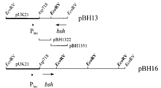
FIG. 4. Plasmid maps of plasmids pBH13 and pBH16, which confer BSH activity, and two subclones. Heavy lines, plasmid pUK21; boldface restriction sites, sites present in the insert; P lac , E. coli lacZ promoter.
