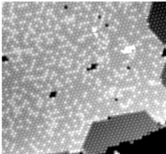
Fig. 1. Monolayer of C 60 on Au(111), the area is 47 × 44 nm 2 , the tunneling current is 13 pA at -1.85 V tip bias.
