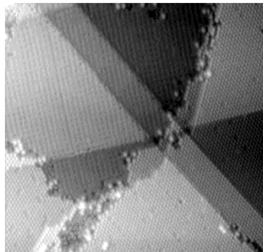
Fig. 3. A mixed layer of CuPc and C 60 at 50 K; the area is 93 × 86 nm 2 , the tunneling current is 10 pA at -2.1 V tip bias, the STM data have been partially shaded to enhance the visibility of small details, the quadratic ordering of the CuPc is visible at the upper left, and to the lower right the hexagonal ordering of the C 60 molecules can be seen.
