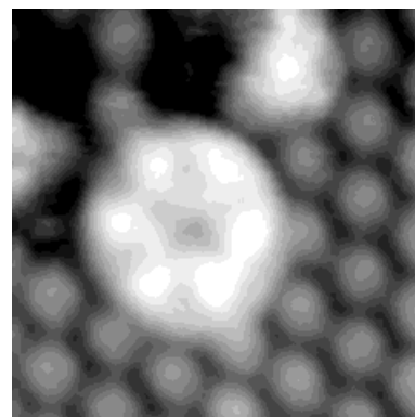
Fig. 7. Individual CuPc molecule on C 60 island of Figure 6, the area is 5.4 × 5.2 nm 2 , the tunneling current is 8 pA at 1.5 V tip bias.
