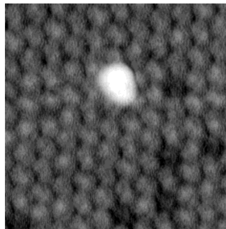
Fig. 8. Individual CuPc molecule at about 50 K; the area is 22 × 22 nm 2 , the tunneling current is 13 pA at 2 V tip bias.
