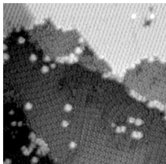
Fig. 4. Smaller area of a mixed layer of CuPc and C 60 at 50 K; the area is 47 × 47 nm 2 , the tunneling current is 24 pA at 1.8 V tip bias, the STM data have been partially shaded to enhance the visibility of small details.
