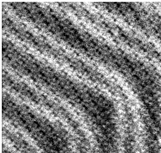
Fig. 2. Monolayer of CuPc on Au(111), the area is 23 × 21 nm 2 , the tunneling current is 9 pA at -2.1 V tip bias.
