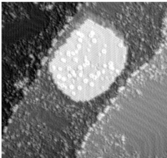
Fig. 5. Mixed layer of C 60 and CuPc for a slightly different preparation; the area is 87 × 80 nm 2 , the tunneling current is 9 pA at 2.1 V tip bias, the domain boundary of the CuPc (lower right) is decorated by C 60 molecules, on top of the C 60 island individual CuPc molecules are found.
