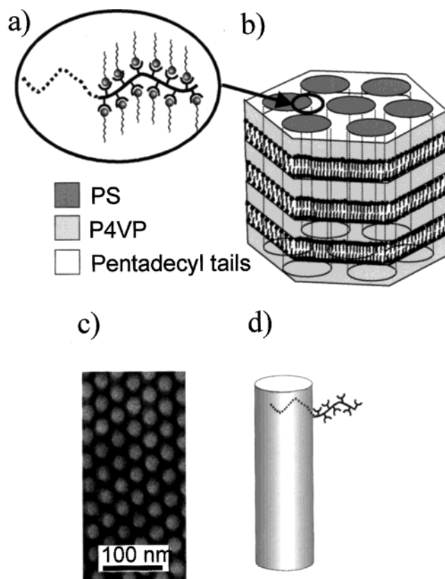
Figure 1. (a) Schematics to form the supramolecular comb-coil diblock copolymer; (b) the initial hexagonally self-organized structure before the removal of the PDP amphiphiles, as demonstrated by SAXS; (c) a transmission electron microscopy picture of the cylindrical structure of a similar supramolecular P4VP(NDP)- b -PS comb-coil diblock copolymer based on a slightly longer amphiphile nonadecylphenol (NDP); 6 (d) Scheme of a fibrillar nano-object.
