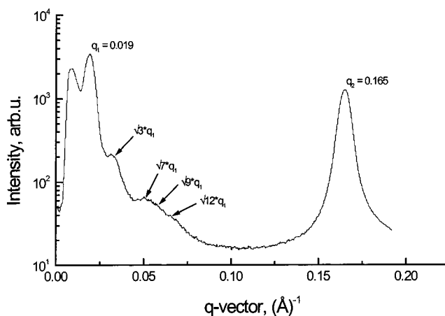
Figure 2. SAXS pattern of P4VP(PDP)-b-PS demonstrating the cylindrical morphology. The position of the first scattering peak corresponds to 2\pi/q^* = 33 \text{ nm} . Also present is the main scattering peak of the short length scale lamellar structure of the P4VP(PDP) matrix.
