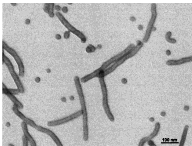
Figure 4. STEM picture of cylindrical aggregates of P4VP-(20.7)-b-PS(21.4k) diblock copolymers stained with iodine for 2.5 h.
