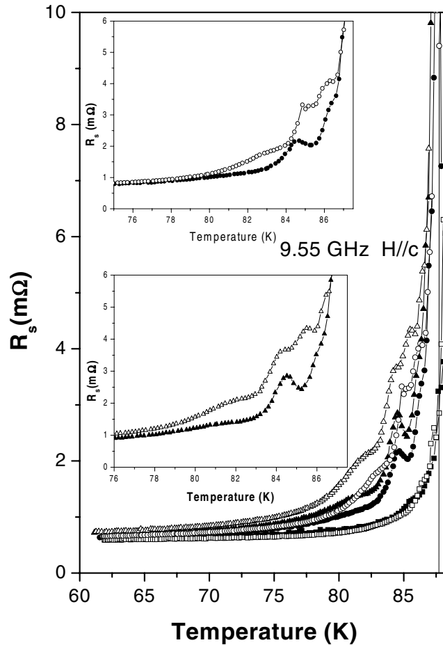
Figure 2. R_s vs. T plots at 9.55 GHz for various applied fields ( \parallel c ) for both pristine (filled points) and irradiated (open points) films. The two insets separately show R_s vs. T plots for 0.4 T (upper) and 0.8 T (lower).
