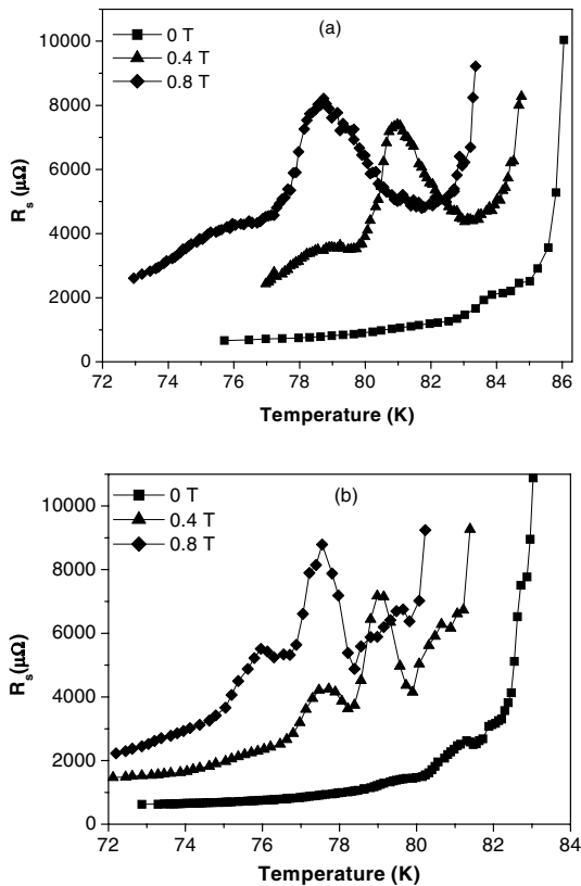
Figure 2. Plot of R_s vs. temperature at different applied magnetic fields at frequency 9.55 GHz, where (a) and (b) are for samples S_1 and S_2 respectively.
