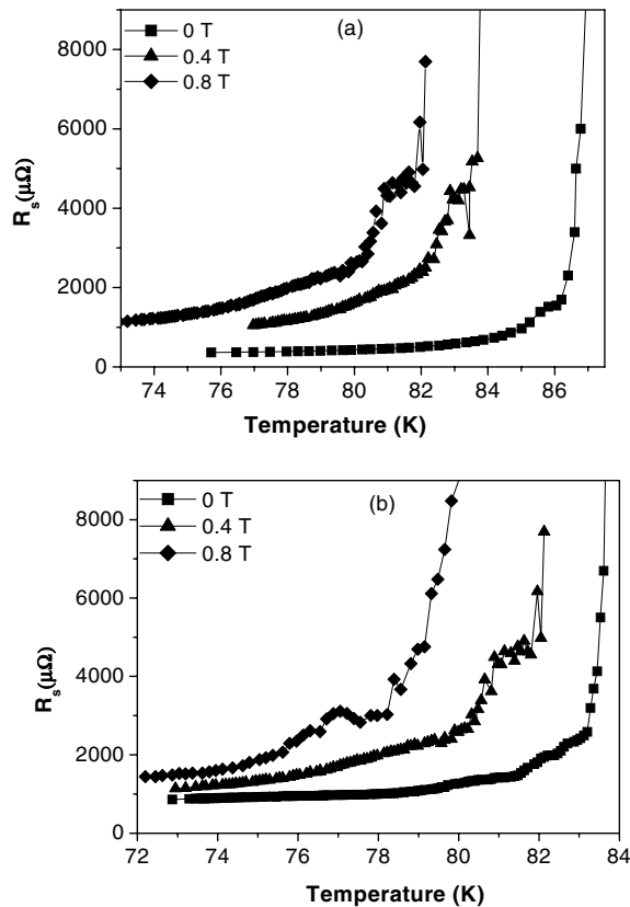
Figure 1. Plot of R_s vs. temperature at different applied magnetic fields at frequency 4.88 GHz, where (a) and (b) are for samples S_1 and S_2 respectively.
