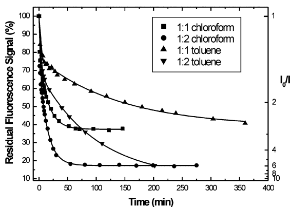
Fig. 3 Fluorescence intensity of 1:1 and 1:2 OPV 2 UP 2 :C 60 -UP 2 mixtures in chloroform and toluene together with the exponential decay curves. I_0 represents the fluorescence intensity of the pure OPV 2 UP 2 solution, whereas I indicates the OPV 2 UP 2 fluorescence in the indicated mixture. The concentration of OPV 2 UP 2 is 5 \times 10^{-7} M, \lambda_{\text{exc}} = 435 nm, \lambda_{\text{em}} = 494 nm, T = 20 °C.
