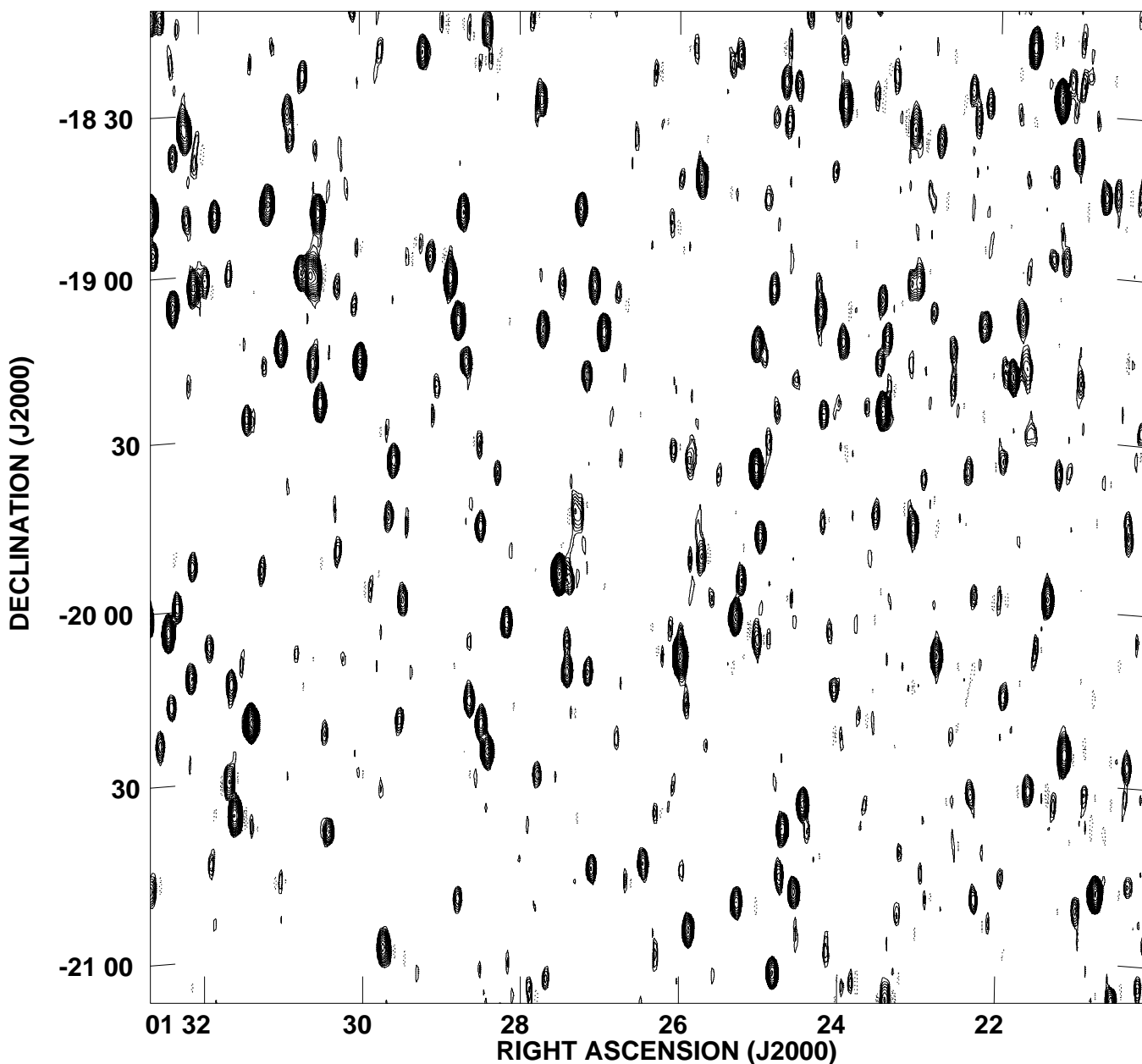
Fig. 2. Central part of the field centered at \alpha = 1^h 28^m , \delta = -20^\circ . The contour scheme is a geometric progression in \sqrt{2} , which implies a factor 2 change in surface brightness every two contours (negative contours are dotted). The first contour is at 3\sigma with \sigma = 2.0 \text{ mJy Beam}^{-1} . Note that even with the elongated beam, we can still resolve several sources.
