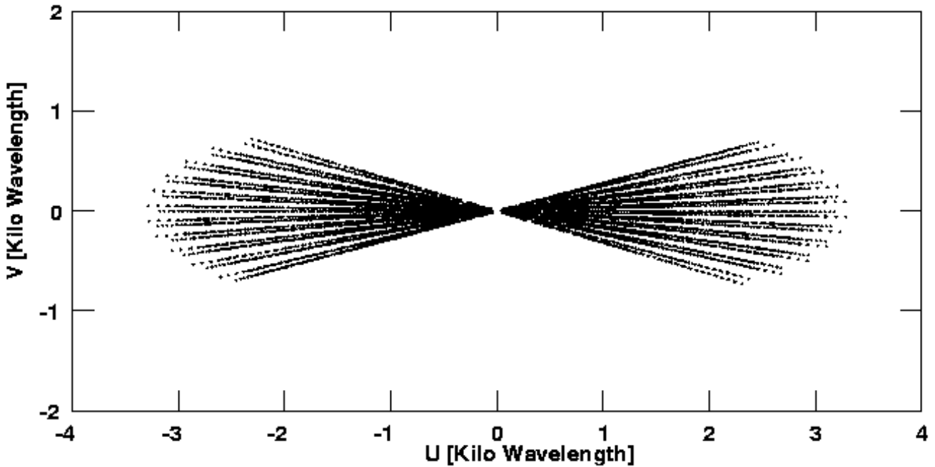
Fig. 1. Sample u - v coverage plot of the field centered at \alpha = 1^h 28^m , \delta = -20^\circ . The v -coverage is limited due to the low declination. Note the excellent radial coverage due to the bandwidth synthesis technique.
