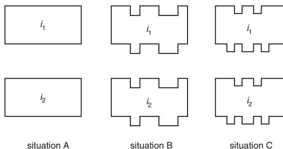
Fig. 5 Graphical representation of variations of having one signature with two implementations
