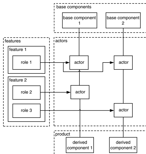
Fig. 1 Conceptual view of feature model
