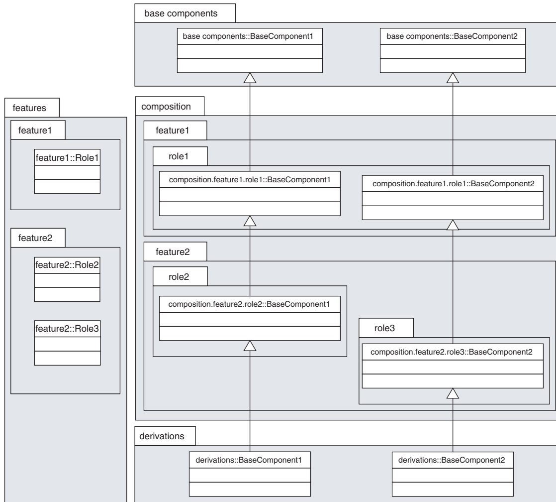
Fig. 6 UML diagram of prototype implementation of Fig. 1
