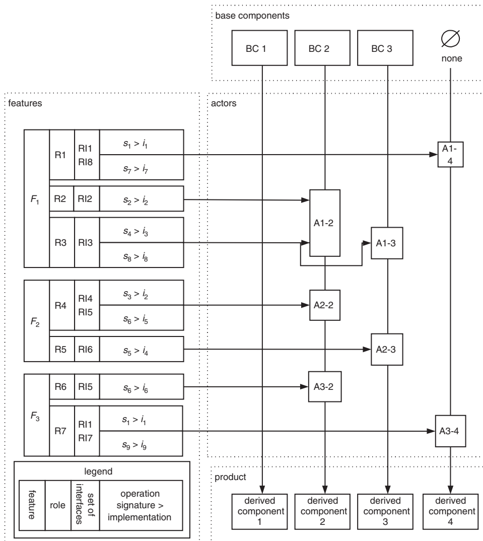
Fig. 3 Graphical representation of feature composition
