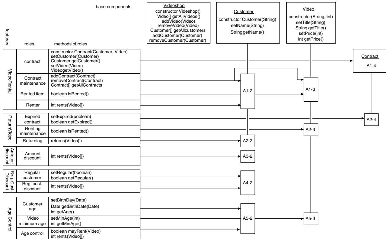
Fig. 2 Features, roles and actors of video shop renting system
