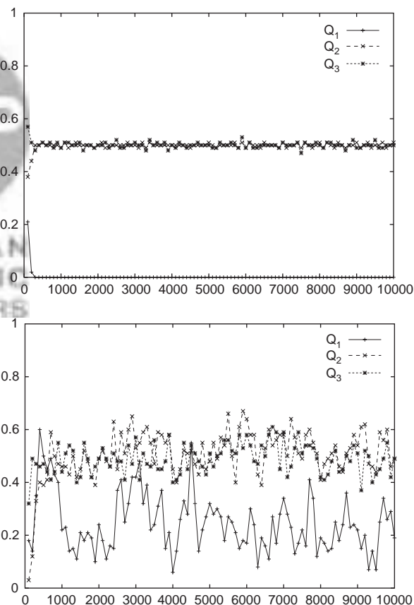
Fig. 8. Event-by-event simulation of Shor's quantum algorithm for factoring the integer N = 15 , using the value a = 7 (see Section 2.5). Each data point represents the average of 100 output events. The parameter that controls the learning process of the DLMs is \alpha = 0.99 . Left: Deterministic simulation employing DLMs. Right: Stochastic simulation employing SLMs.
