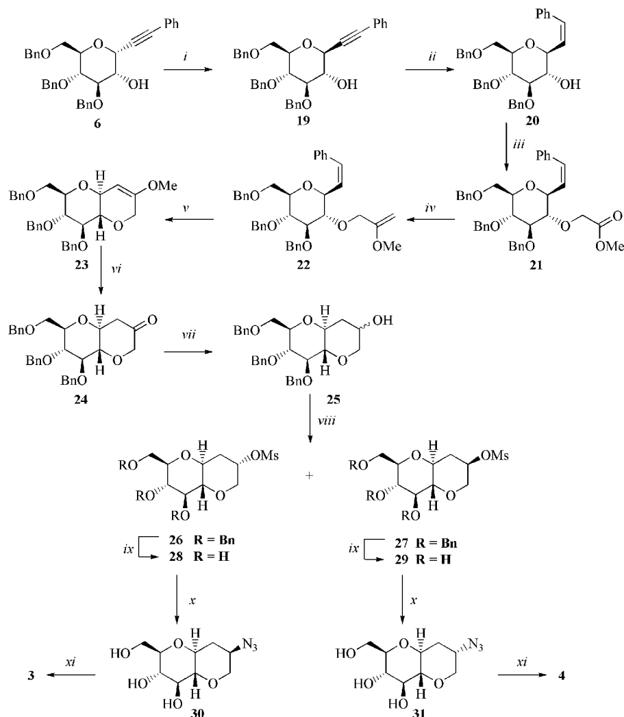
Scheme 2. Reagents and conditions: i ) (a) \text{Co}_2(\text{CO})_8 , \text{CH}_2\text{Cl}_2 , (b) TFOH, \text{CH}_2\text{Cl}_2 , (c) \text{I}_2 , THF, [6] ii ) \text{H}_2 , Lindlar's catalyst, EtOAc, [6] iii ) methyl bromoacetate, TBAI, NaH, DMF, 87%. iv ) \text{Cp}_2\text{TiMe}_2 , THF, 60 °C, 72%. v ) dichlorido(1,3-dimesityl-2-imidazolidinylidene)(phenylmethylene)(tricyclophosphane)ruthenium, \text{CH}_2\text{Cl}_2 , reflux, 86%. vi ) TFA, water, \text{CH}_2\text{Cl}_2 , 90%. vii ) L-selectride, THF, -78 °C to room temp. viii ) MsCl, \text{Et}_3\text{N} , \text{CH}_2\text{Cl}_2 , 0 °C, 26 36%, 27 43%, two steps, ix ) \text{H}_2 , Pd/C, EtOH, 28 quant, 29 95%. x ) \text{NaN}_3 , DMF, 70 °C, 30 70%, 31 74%. xi ) TEMPO, NaOCl, \text{NaHCO}_3 , MeCN, 0 °C, 4 49%, 3 72%.
